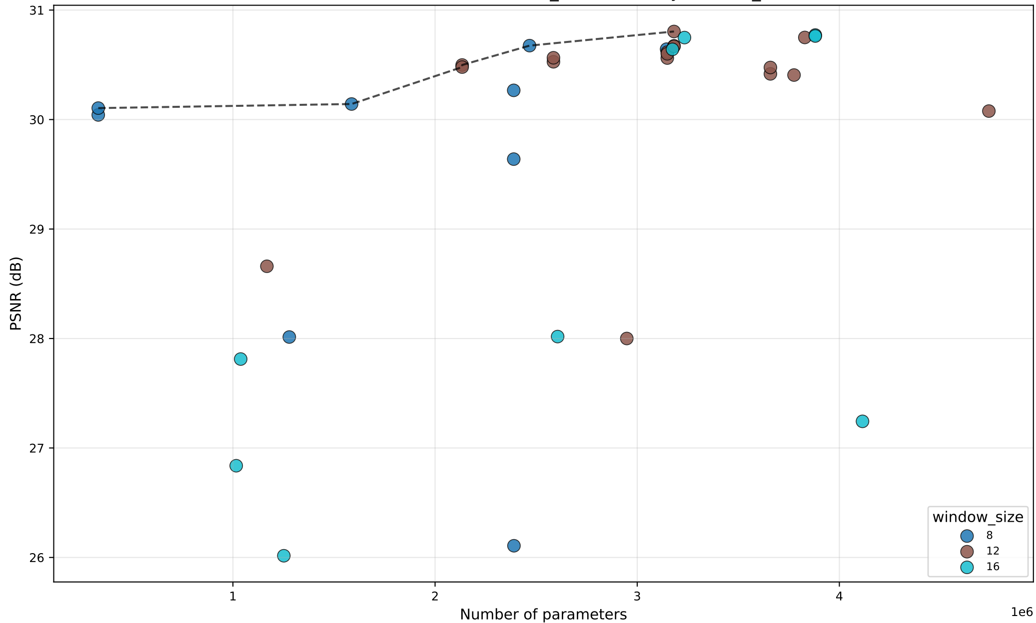
PSNR vs #Params — DHTCUN_baseline — by window_size
